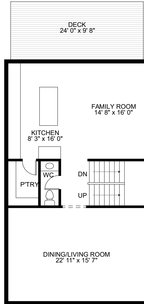
Living Level
