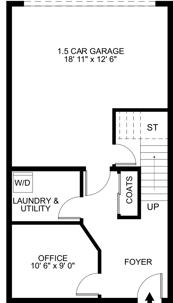
Garage Level
